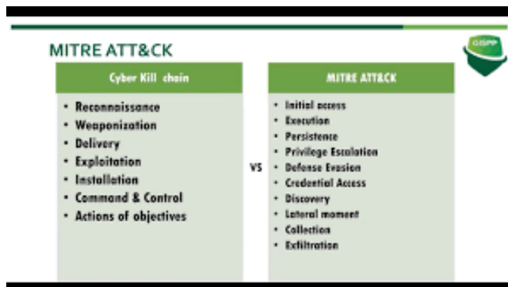
Figure 5: Comparison between Cyber Kill Chain and MITRE ATT&CK (Adopted from YouTube)
