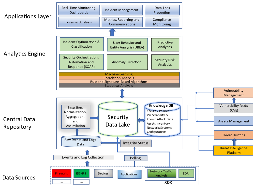
Figure 9: The proposed solution architecture for the security operations center
