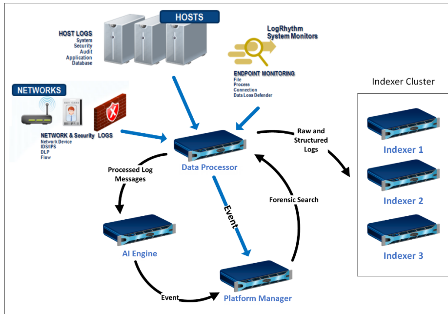
Figure 7: LogRhythm SOC architecture
